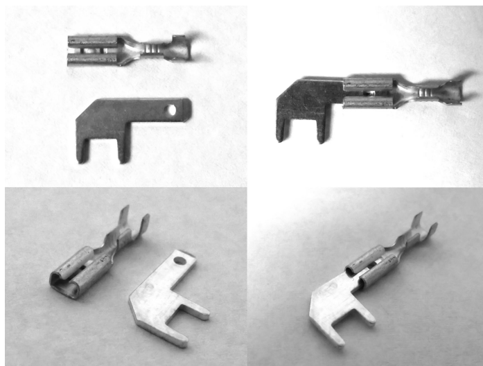
Obr. 1 – FASTON konektory
