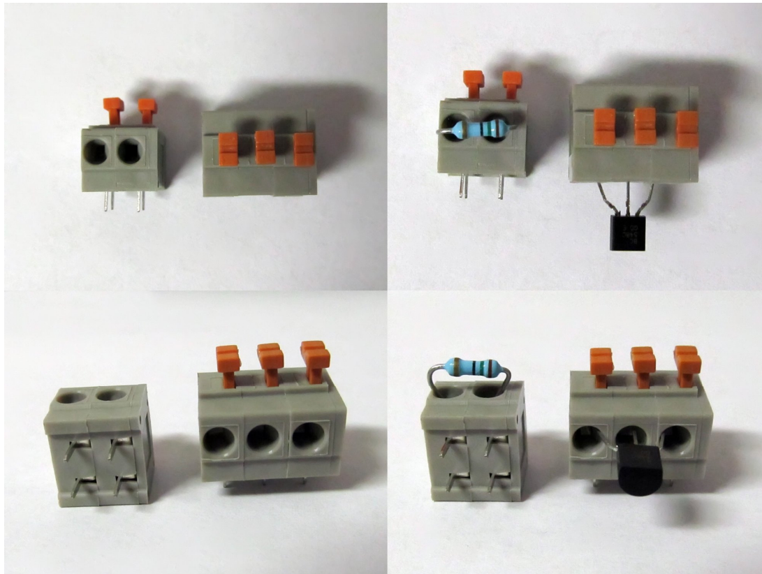
Obr. 2 – Svorkovnice ARK124A/2 a ARK124A/3
